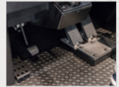
Throttle and retarder/service brake pedals matching OEM machine
